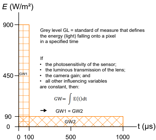
Grey level at various values for exposure time and irradiance
