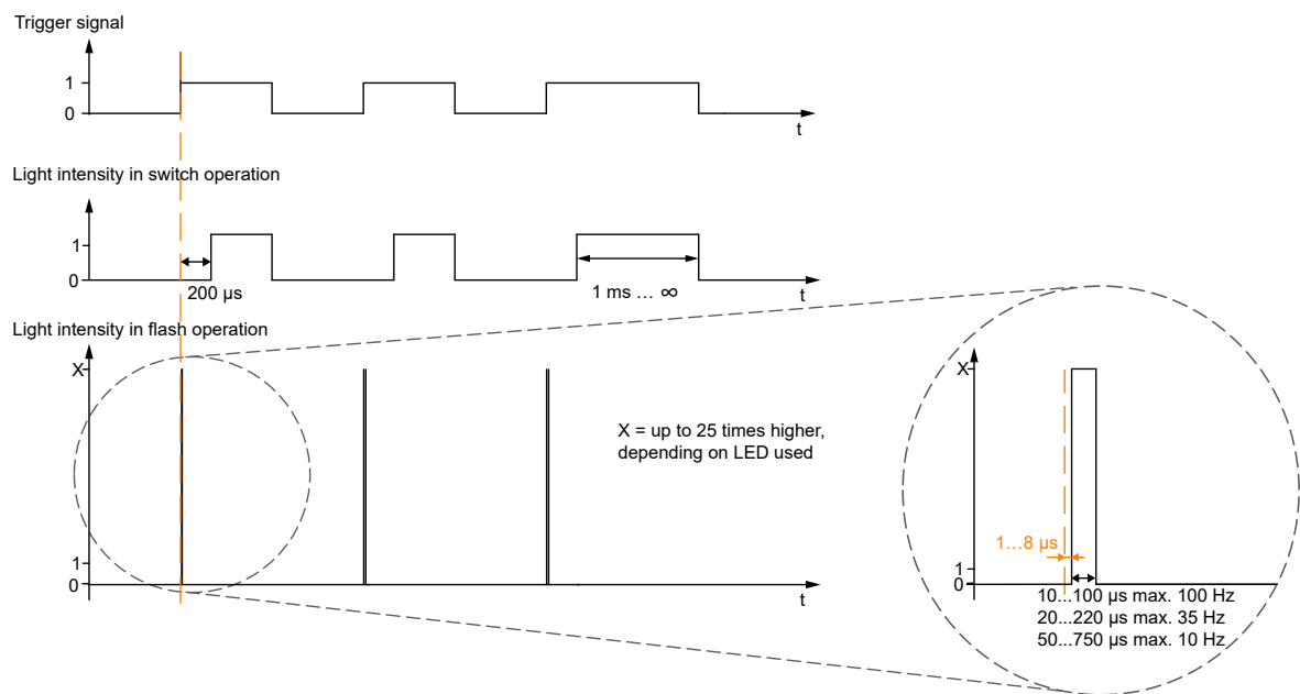
Comparison of pulse and strobe mode lighting
