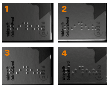
Shape-from-shading image capture using 4 miniature bars from the LSB series
